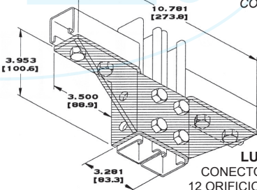
LU-2228 CONECTOR DE 3 ALAS 9 ORIFICIOS NINE HOLE TRIPLE WING CONNECTION
